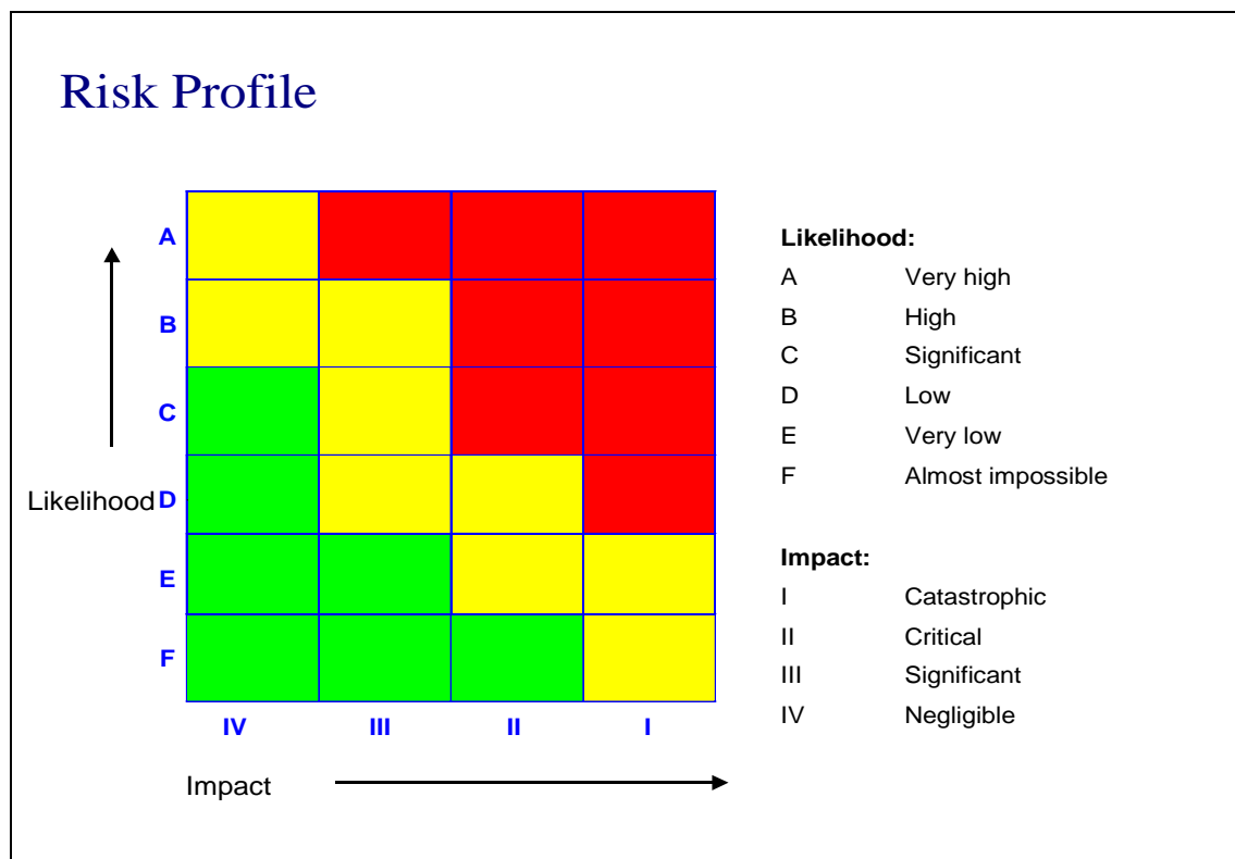
Figure 4: Risk Matrix
